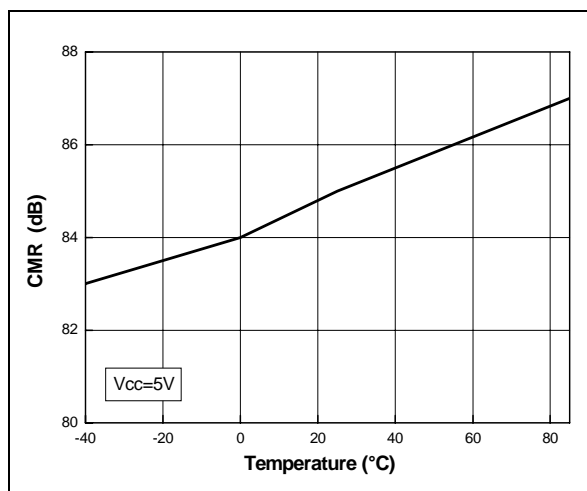
Figure 22. CMR vs. temperature
